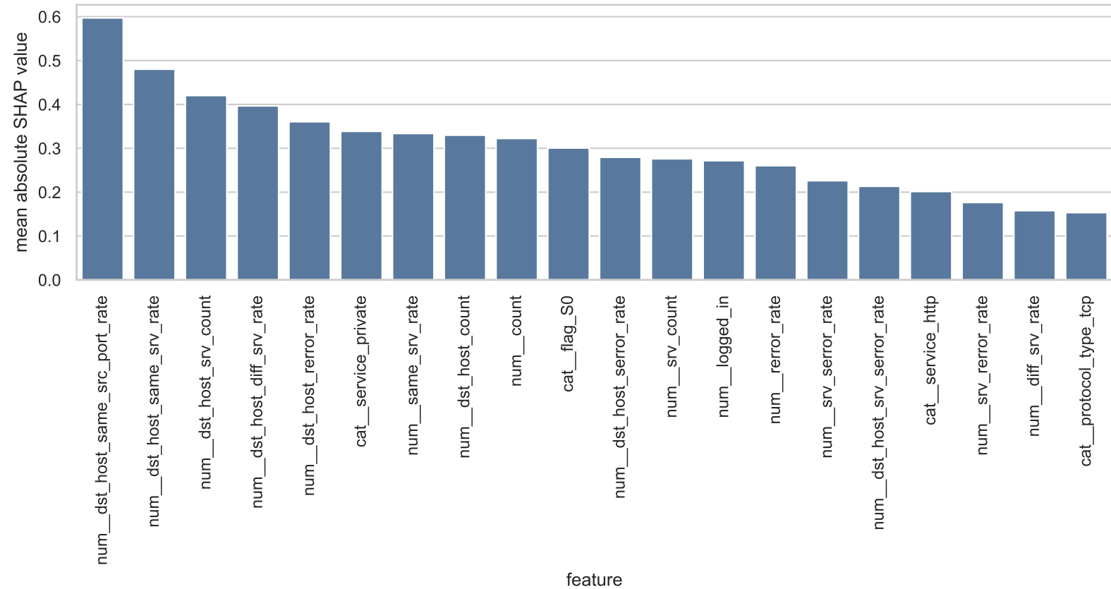
attack: Mean Absolute SHAP Values
